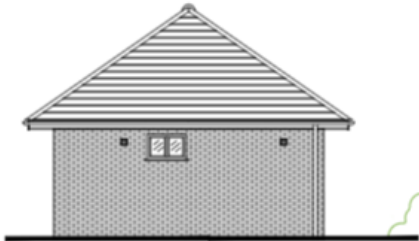
EXISTING EAST ELEVATION 1:50
